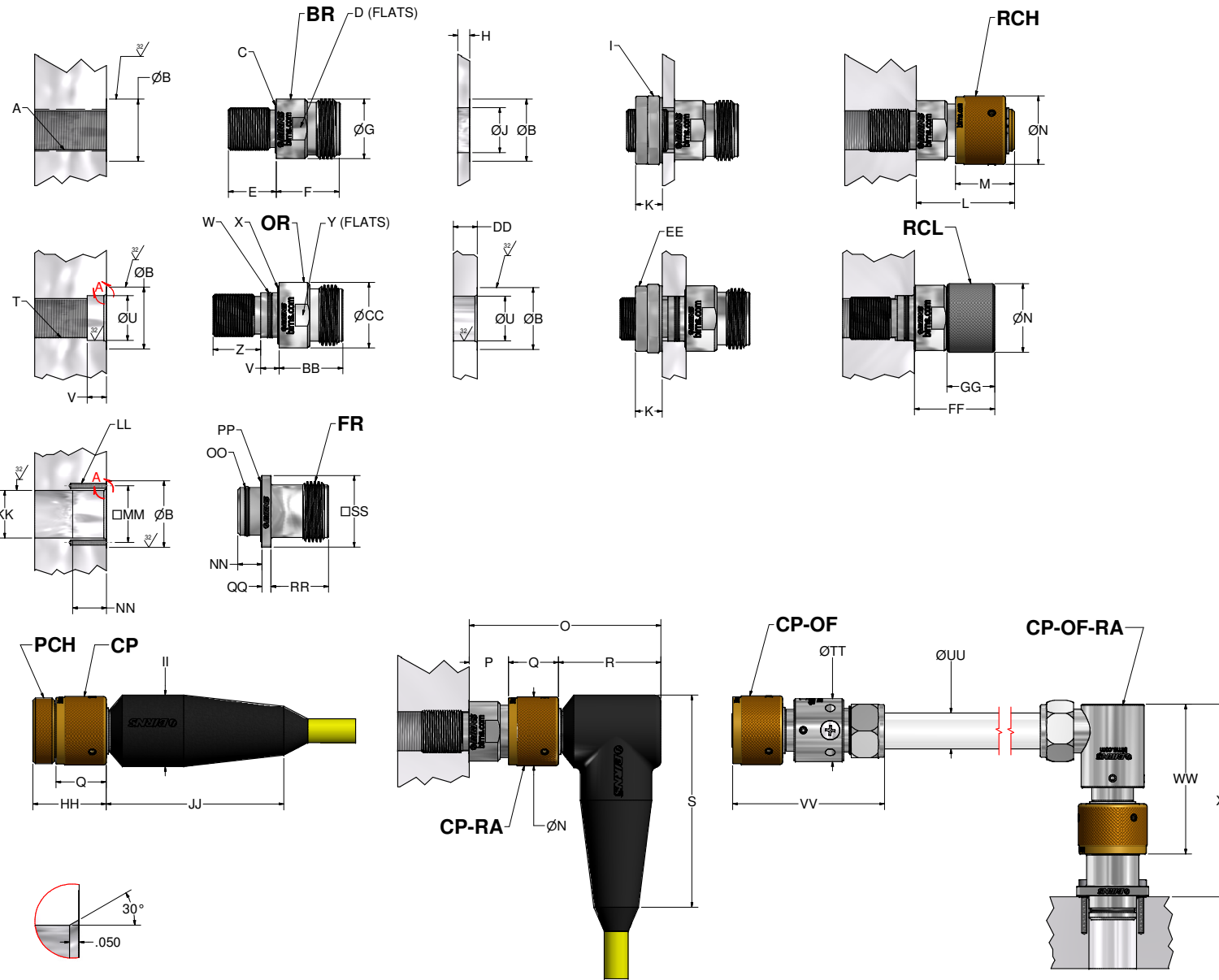
DETAIL A TYPICAL O-RING LEAD IN
